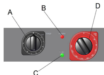
Figure 1 Control panel
