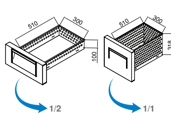
Raf ve Raf Kızağı / Shelf and Shelf Holder
